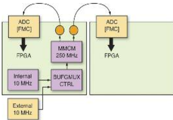
Figure 4: The two FPGA boards must be precisely synchronous. The clocking scheme shown here ensures that they are.
