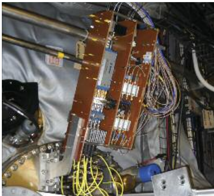
Figure 3: The RF electronics connected to the MAST tokamak downconvert the incoming 6 to 40 GHz signal to the 250 MHz bandwidth signal the FPGA data acquisition box will process.
