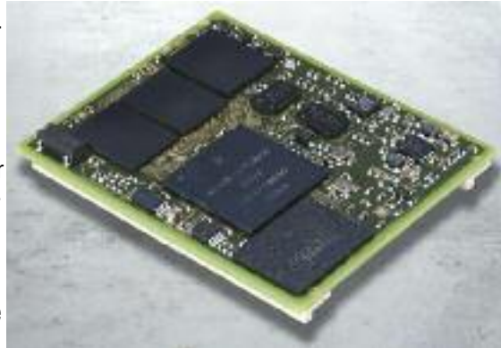
TQ ARM11 module with Freescale i.MX35 processor
